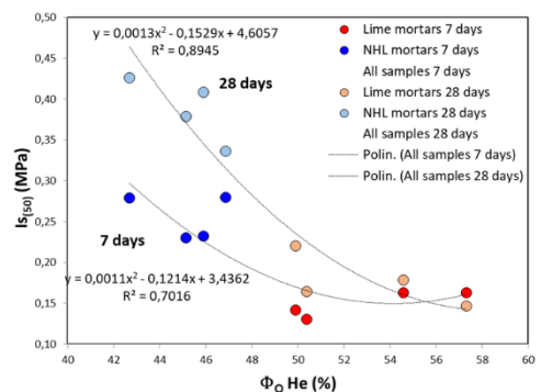
Figure 6 Helium open porosity against puncture resistance index I_{s(50)} .
