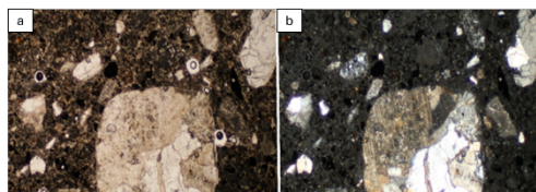
Figure 2. Photomicrographs of MCM01 lime mortar in nicols // (a) and nicols X (b) (2.5x). Detail of the silicate aggregate (quartz and feldspar).
